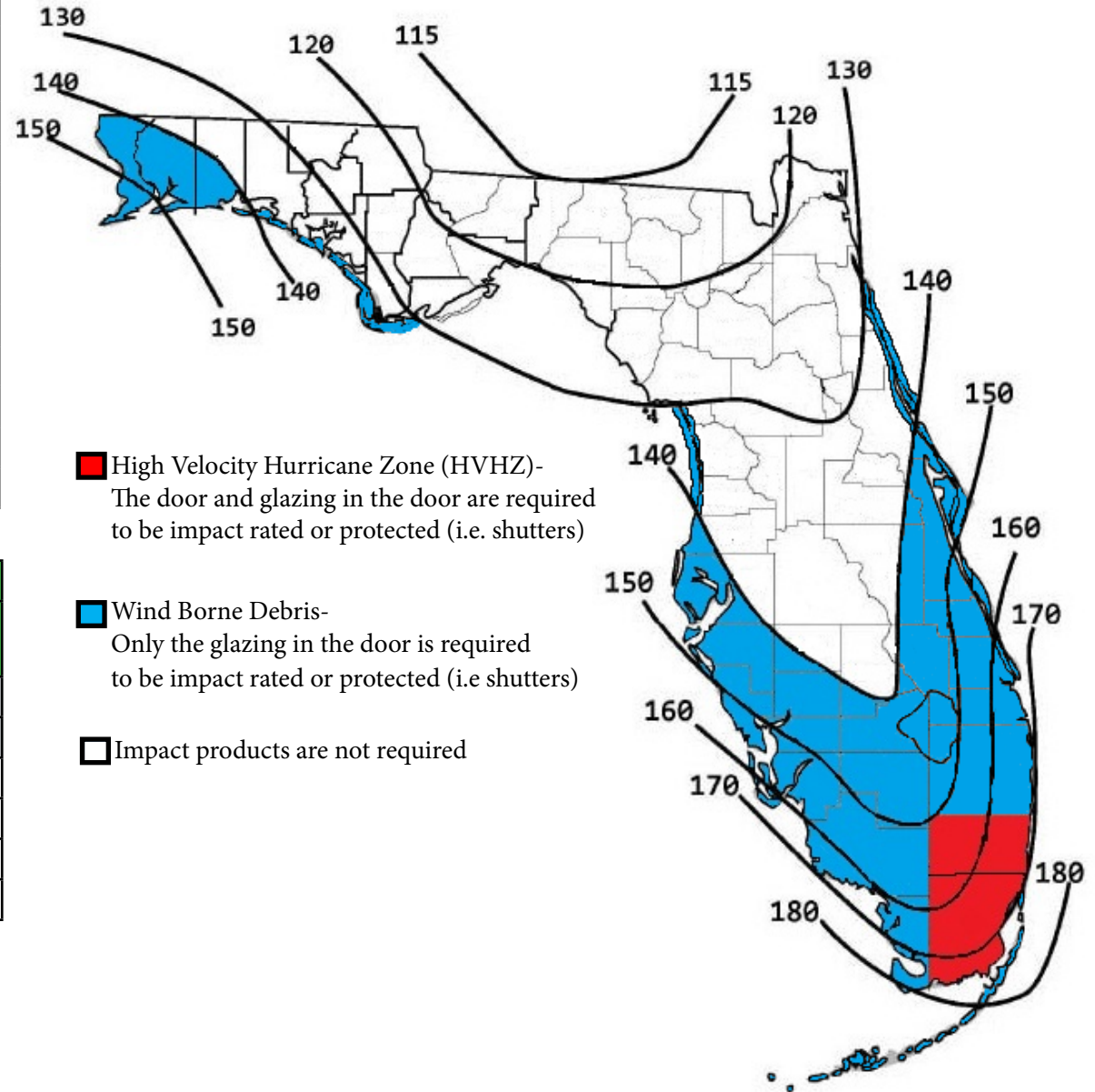
Residential Wind Speed Map (Risk Category 11)
